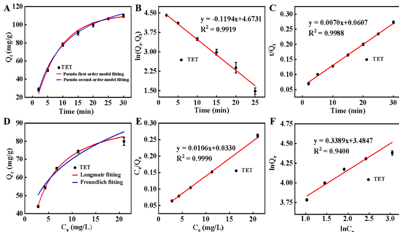
Fig. 5. (A) Adsorption of TET fitted by using pseudo-first-order and pseudo-second-order kinetic models. TET solution: 20 \mu\text{g/mL} ; apt-TMNzyme: 50 \mu\text{g/mL} , pH 9.0, adsorption time: 30 min. The pseudo-first-order kinetic (B) and pseudo-second-order kinetic (C) isotherm fittings for TET on apt-TMNzyme. (D) The effect of TET initial concentration on apt-TMNzyme by the adsorption isotherm. The fitting curves of Langmuir model (E) for TET and Freundlich model (F) on apt-TMNzyme.
