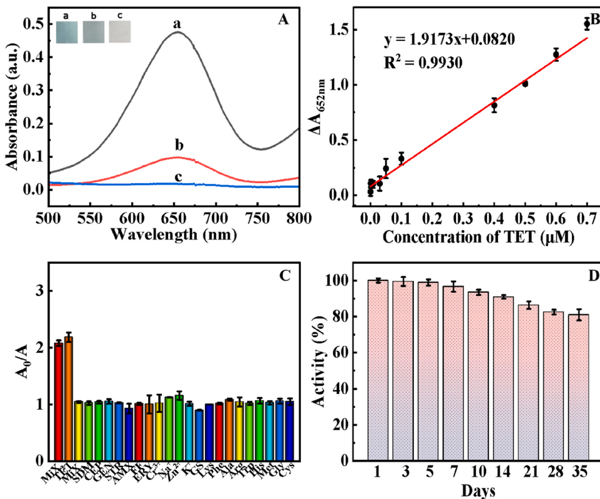
Fig. 3. (A) The absorbance of the catalytic reaction system with the addition of TET (inset (a): apt-TMNzyme + H 2 O 2 + TMB + Buffer, (b): apt-TMNzyme + H 2 O 2 + TMB + TET (0.1 mM) + Buffer (c): apt-TMNzyme + H 2 O 2 + TMB + TET (0.3 mM) + Buffer). (B) The linear calibration plots for the quantitative determination of TET ( \Delta A = A_0 - A , where A_0 and A are the absorbance of the reaction system without and with TET). (C) Selectivity determination of apt-TMNzyme colorimetric sensor for TET. (D) The stability of POD-like activities for apt-TMNzyme five weeks.
