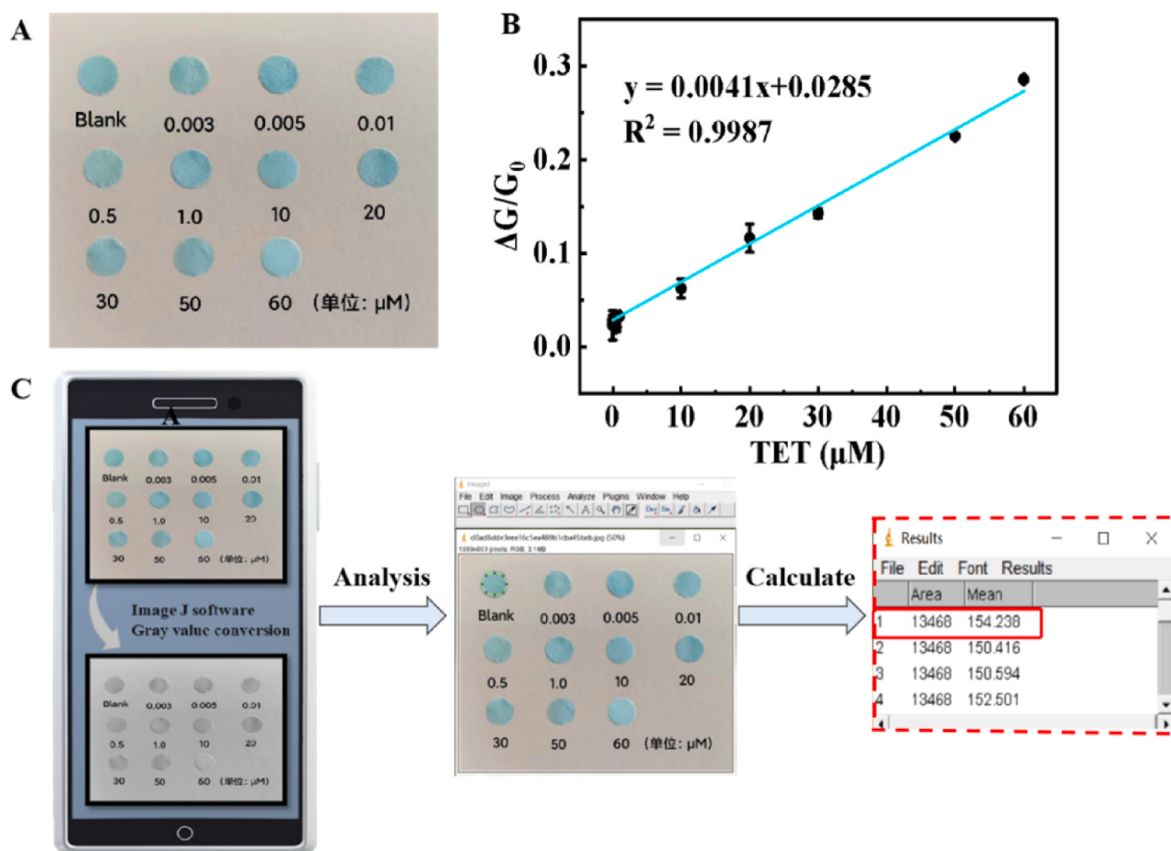
Fig. 4. (A) Colorimetric images of test papers after the reaction with different concentrations of TET (0, 0.003, 0.005, 0.01, 0.5, 1.0, 10, 20, 30, 50, 60 \mu\text{M} ); (B) Linear relationship between \Delta G/G_0 values and TET concentrations (0.003–60 \mu\text{M} ). (C) The schematic diagram of TET detection by the designed smartphone.
