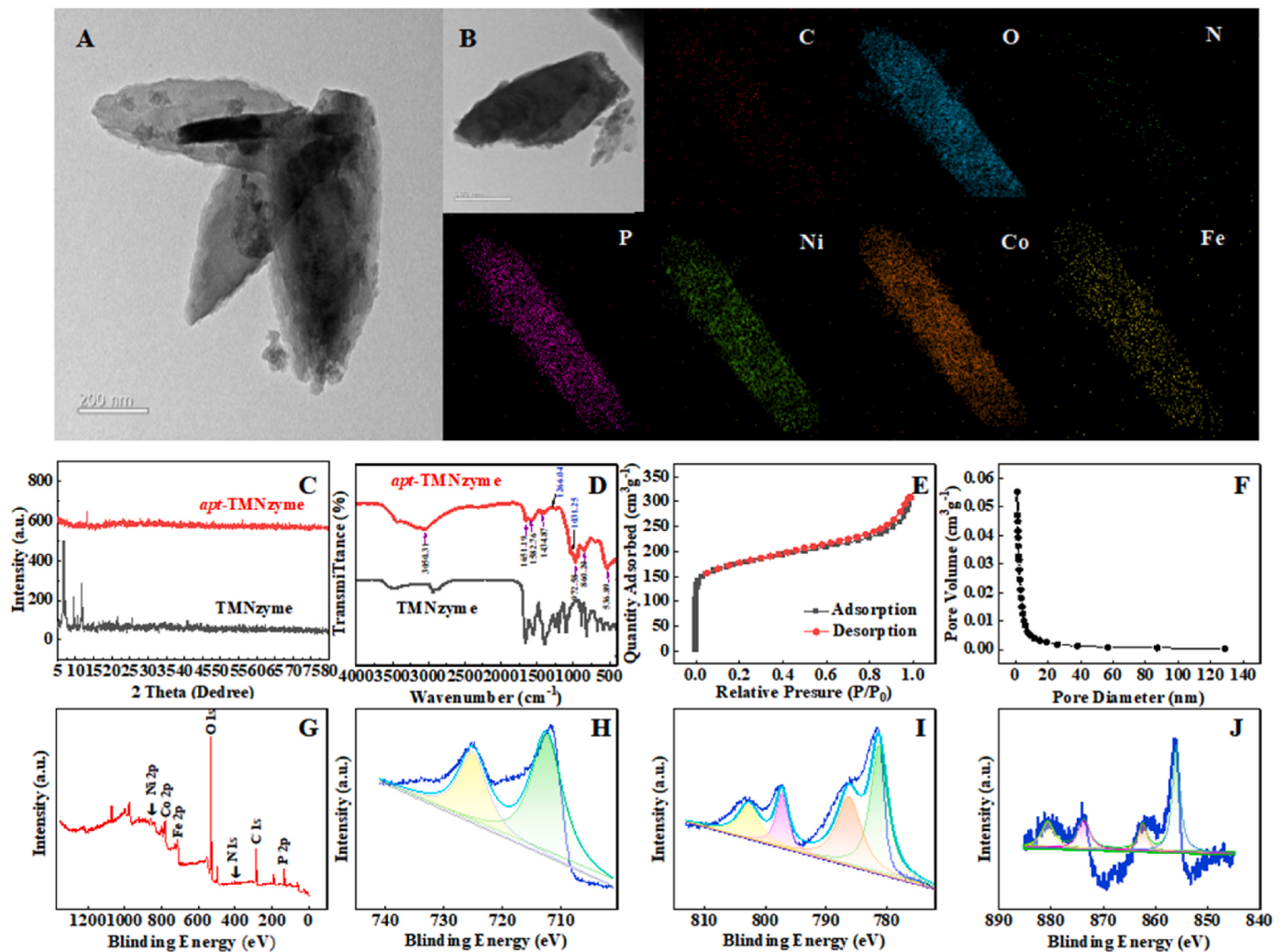
Fig. 1. (A) HR-TEM image of apt -TMNzyme and (B) corresponding elemental mappings showing the hierarchical elemental distributions of Ni, Co and Fe. (C) XRD patterns of TMNzyme and apt -TMNzyme. (D) FTIR measurements of TMNzyme and apt -TMNzyme. (E) N_2 adsorption/desorption isotherms and (F) the corresponding pore size distribution curve of the apt -TMNzyme. (G) XPS spectra of apt -TMNzyme and high-resolution spectra of Fe 2p (H), Co2p (I) and Ni 2p (J).
