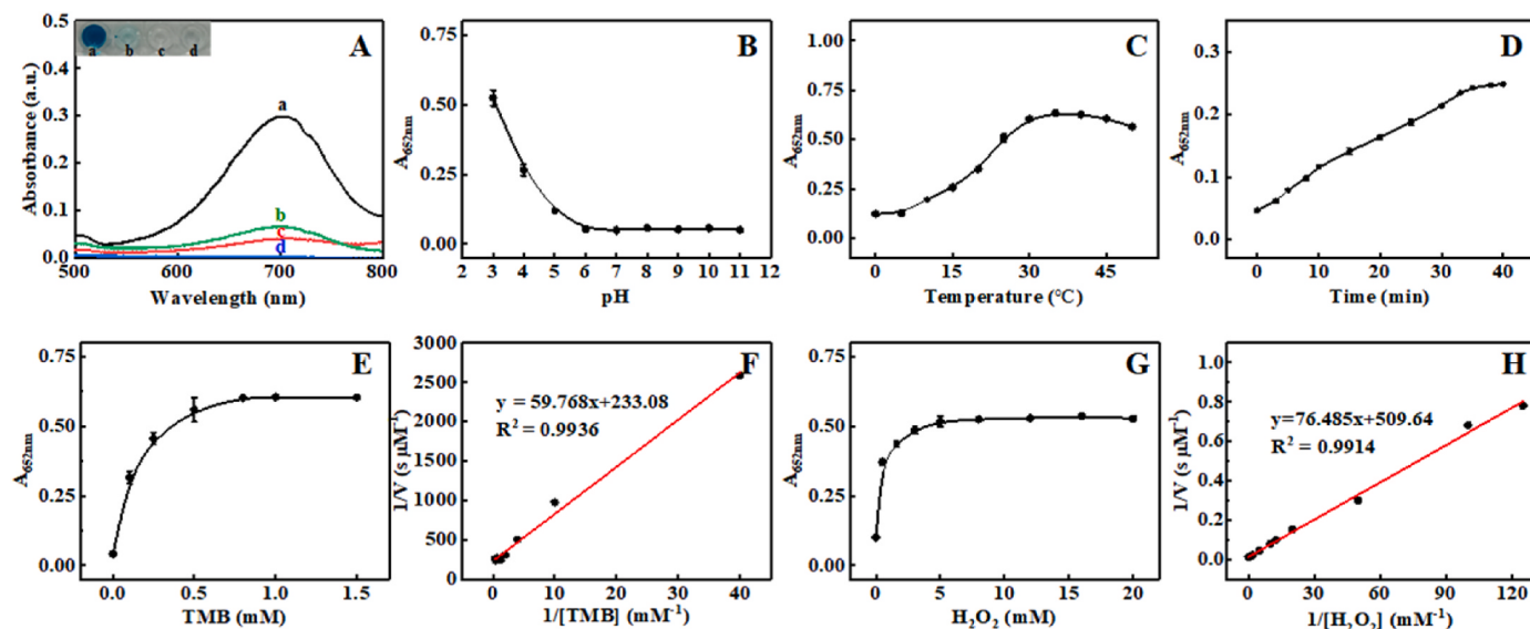
Fig. 2. (A) POD-like activity: typical absorption spectra of TMB, oxidation catalyzed by apt -TMNzyme and control groups in the presence of \text{H}_2\text{O}_2 at pH 4.0, and corresponding color changes (inset (a): apt -TMNzyme + \text{H}_2\text{O}_2 + TMB + Buffer, (b): \text{H}_2\text{O}_2 + TMB + Buffer, (c): apt -TMNzyme + \text{H}_2\text{O}_2 + Buffer, (d): apt -TMNzyme + TMB + Buffer). The effect of pH 3–11 (B), temperature (0 °C–50 °C) (C), reaction time (0–40 min) (D) on the POD-like activity. (E) The concentration of \text{H}_2\text{O}_2 was 10 mM and the TMB concentration varied and (F) Double reciprocal plots of the Michaelis-Menten equation from the activity data of the concentration of TMB. (G) The concentration of TMB was 0.5 mM and the \text{H}_2\text{O}_2 concentration varied and (H) Double reciprocal plots of the Michaelis-Menten equation from the activity data of the concentration of \text{H}_2\text{O}_2 .
